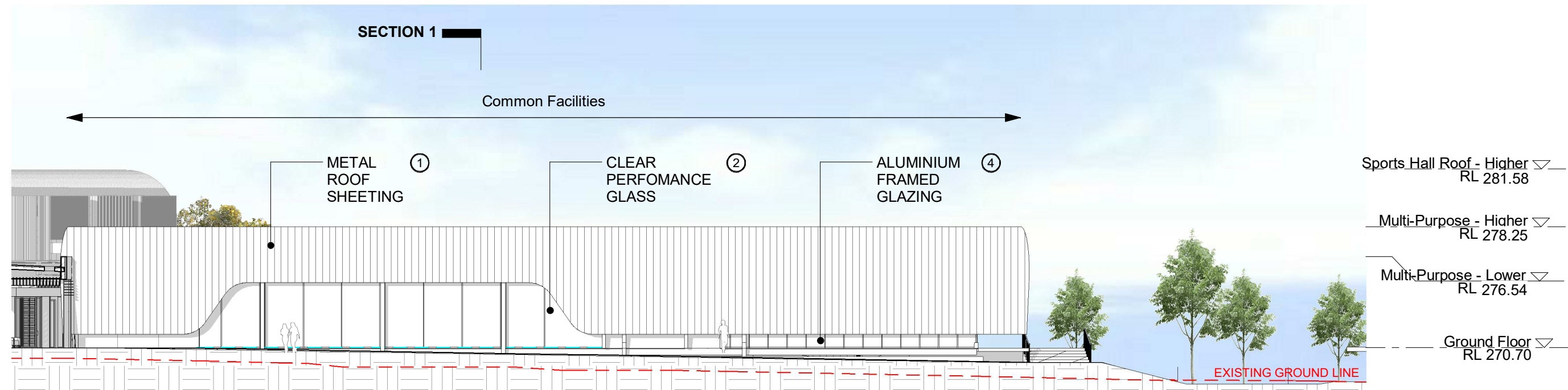
1 East Elevation - Common Facilities 1 : 250
