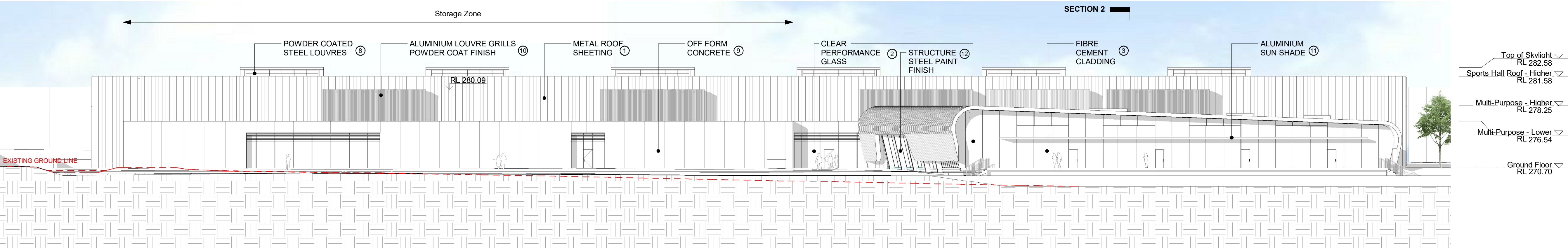
2 North Elevation 1 : 250
