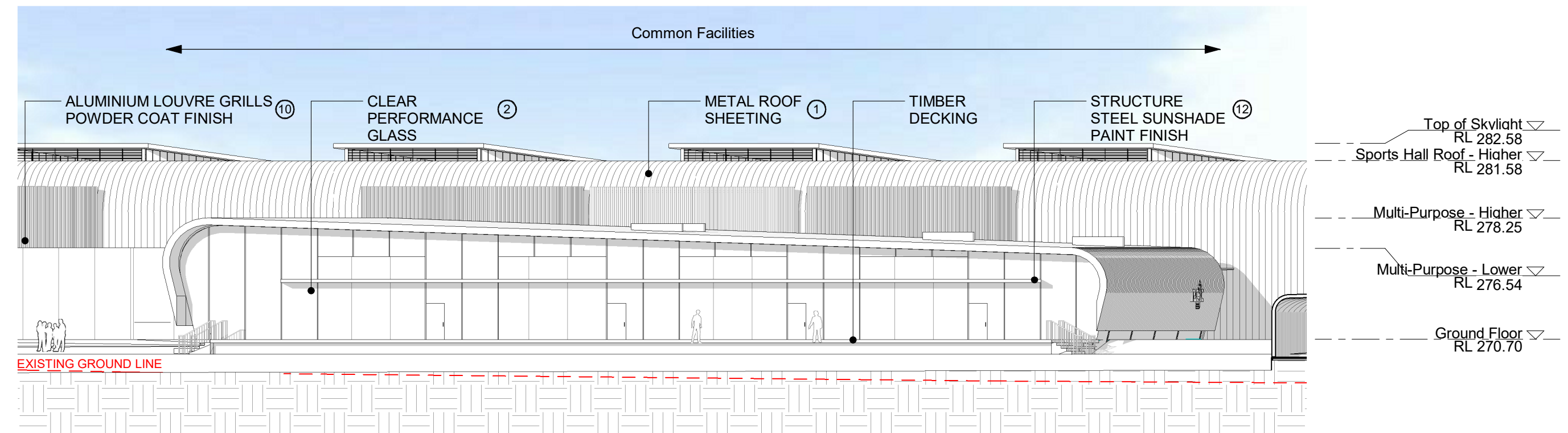
2 North Elevation - Common Facilities 1 : 250
