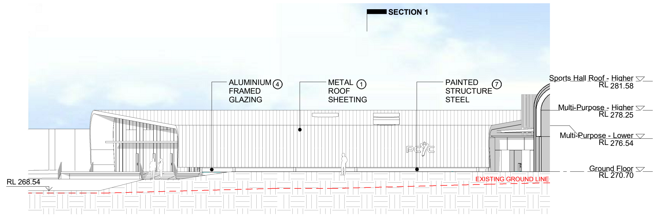
3 West Elevation - Common Facilities 1 : 250
